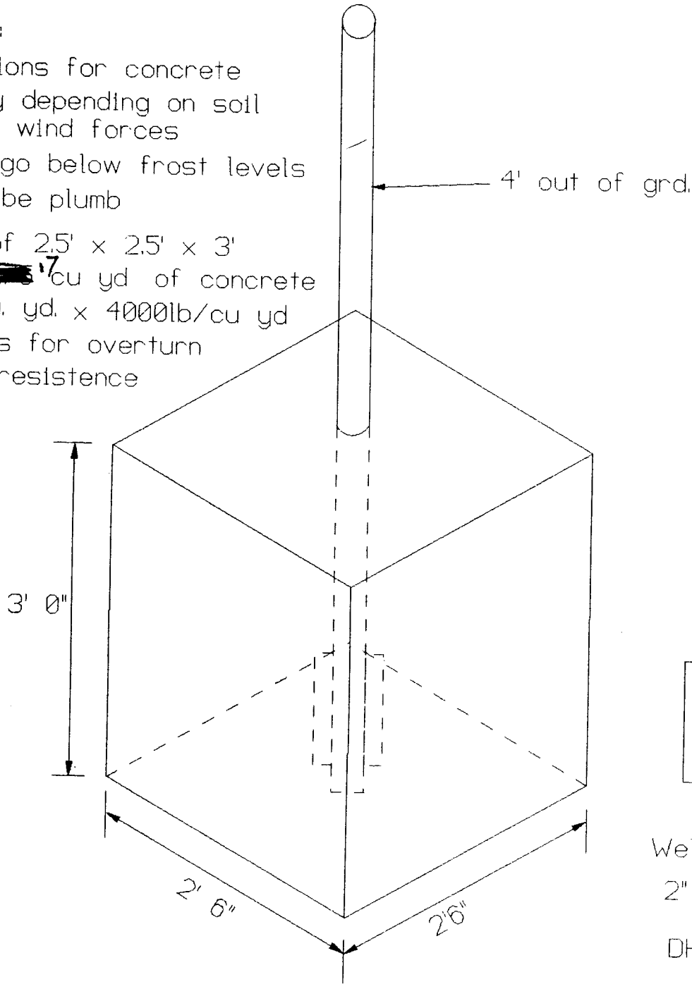
Conc. Pad for 2.4m Antenna
